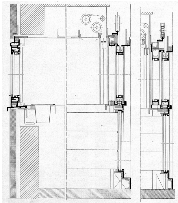
Figure 7. Vertical Section of the Office Windows (Il palazzo 1938).
