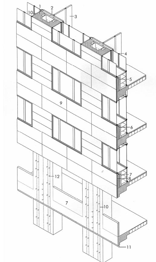
Figure 10. Part Elevation of one of Side Volumes. 1. reinforced concrete structure 2. masonry wall 3. moveable partition 4. aluminium window 5. pumice sheet 6. air space 7. reinforced concrete parapet 8. mortar layer 9. stone slab 10. steel bar 11. stainless steel angle 12. annealed brass stone anchor (drawing by author)
